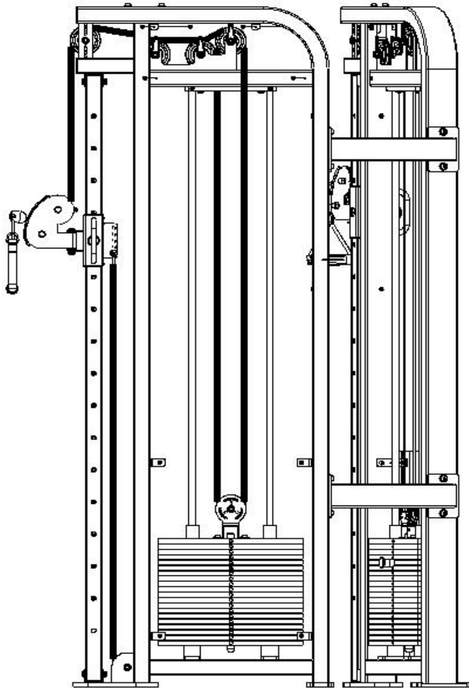
Wire rope alignment diagram
